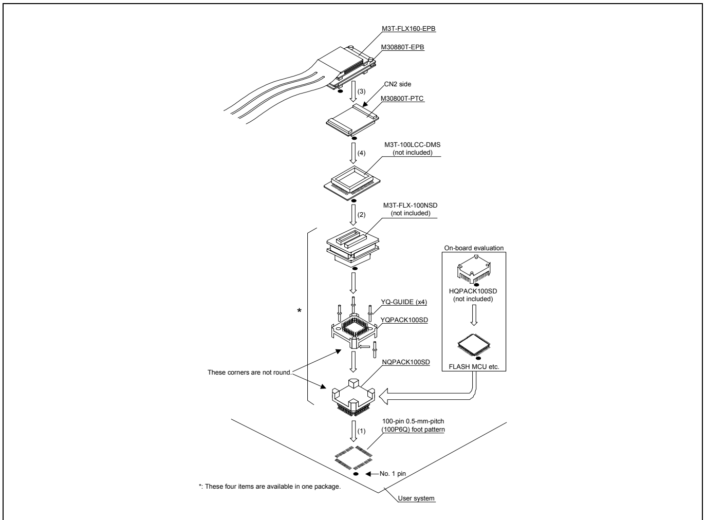
Figure 2.13 Connecting to a 100-pin 0.5-mm-pitch foot pattern (2/3)
